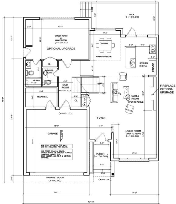
Main Floor with Guest Room
